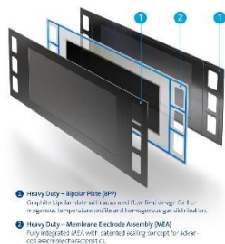
Single Cell of a Heavy Duty Fuel Cell Stack
